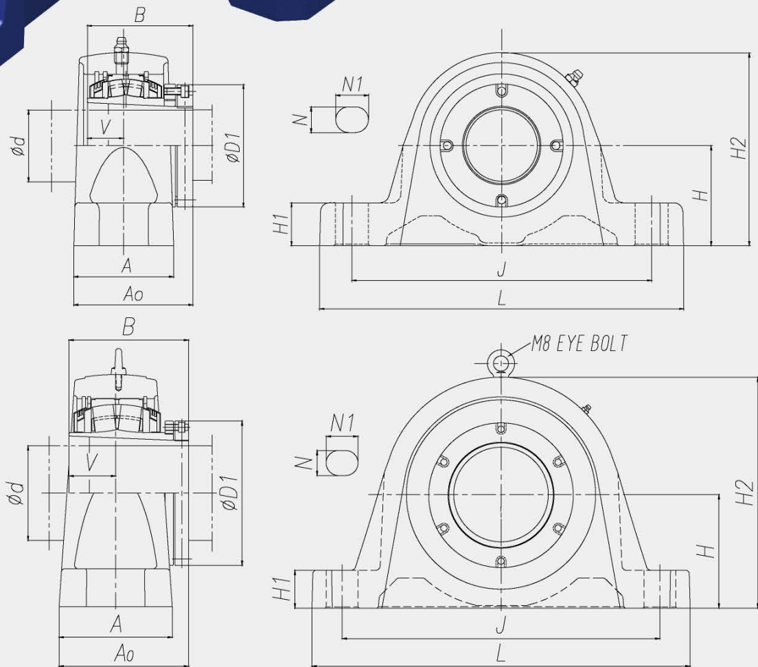
CX2SN28-125 – CX2SN32-140
